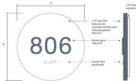
ROOM NUMBER PART# CAM-1000
