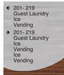
10 LINE DIRECTIONAL SIGN PART# FFI-1118 12" x 14.625"
