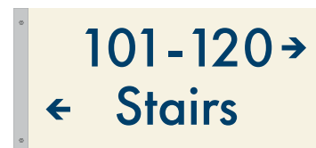
PERPENDICULAR (FLAG) DIRECTIONAL SIGN PART# CLP-1111-L 15.75" x 7.5"
